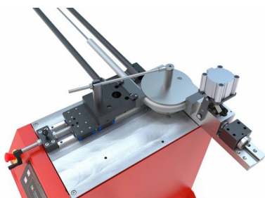
With device AB-CTA for tube bending with mandrel and pneumatic vice
