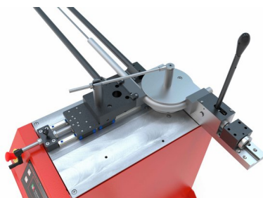
With device AB-CTA for tube bending with mandrel and manual vice
