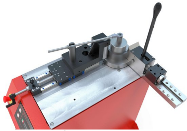
With device AB-CF for round bending
