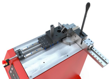
With device AB-PF for angle bending
