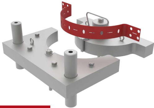
Bracket bender
