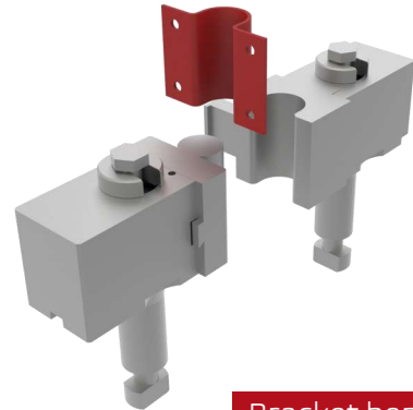
Bracket bender
