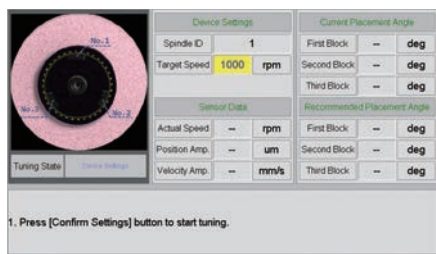
In-Machine Dynamic Balancing
