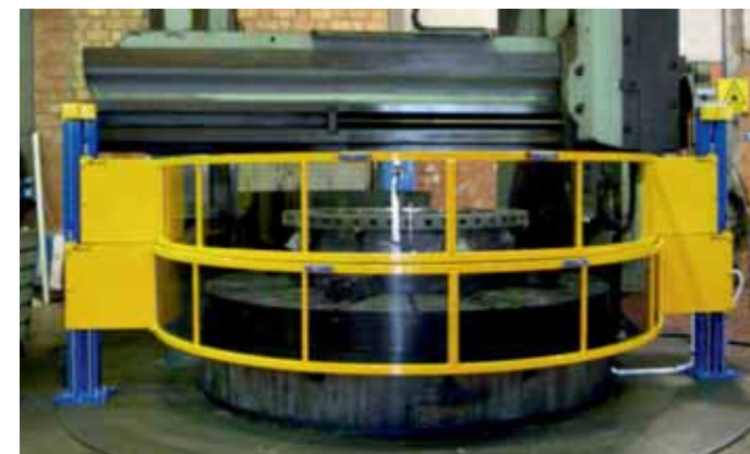
SAFETY GUARDS FOR VERTICAL LATHES
